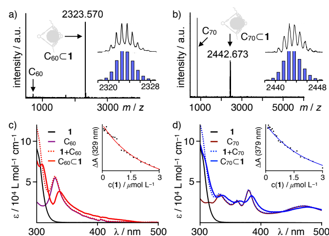
Fig. 2. MALDI-TOF MS (TCNQ, \text{CHCl}_3 ) for 1:1 mixtures of 1 and a) \text{C}_{60} and b) \text{C}_{70} (insets show comparison of measured and simulated isotope patterns); UV/Vis titration experiments for complex formation between 1 and c) \text{C}_{60} (black 1 , purple \text{C}_{60} , dotted red 1 + \text{C}_{60} , red \text{C}_{60}\text{C}1 derived from global fit to 1:1 model, inset shows fit to 1:1 model at \lambda = 329 \text{ nm} ) and d) \text{C}_{70} (black 1 , brown \text{C}_{70} , dotted blue 1 + \text{C}_{70} , blue \text{C}_{70}\text{C}1 derived from global fit to 1:1 model, inset shows fit to 1:1 model at \lambda = 379 \text{ nm} ).
