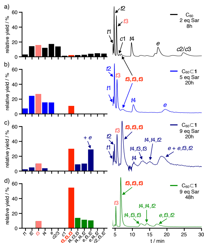
Fig. 5. Relative yields (left, calculated from HPLC profiles) for bisadducts 3 and trisadducts 4 and HPLC chromatograms (right) for a) control experiment with C_{60} (2.0 eq. Sar, 8h)
