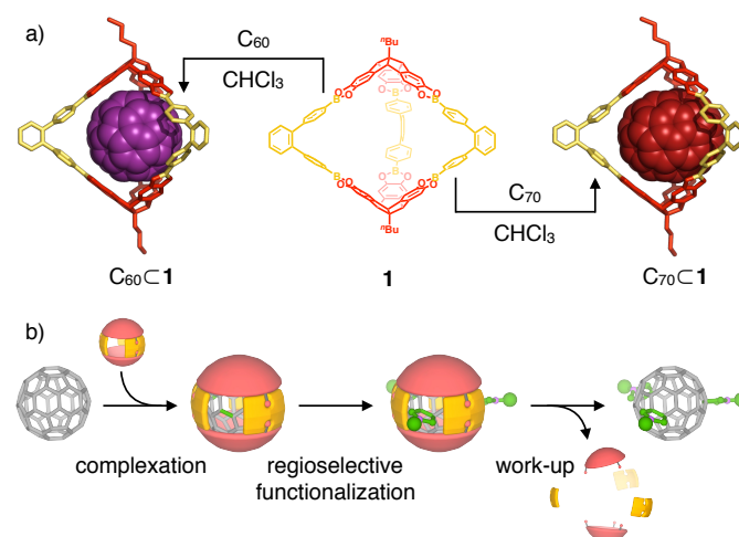
Fig. 1. a) Supramolecular complexation of fullerenes C 60 and C 70 within the cavity of covalent organic boronate ester cage 1 (molecular structures of inclusion complexes are derived from semiempirical PM6 modeling); b) schematic representation for the use of C 60 -cage complexes as shadow masks for a regioselective exohedral C 60 functionalization.
