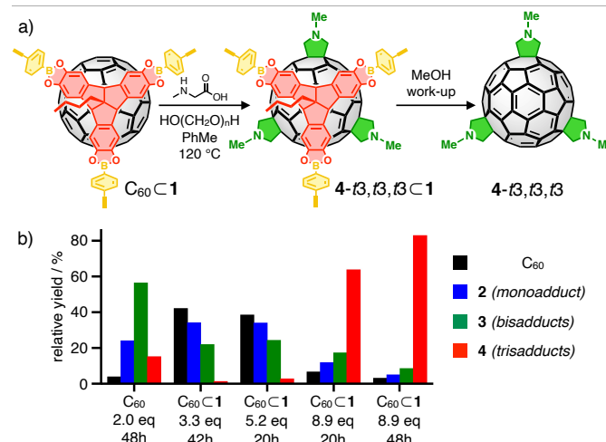
Fig. 4. a) Cage-templated synthesis of N -methylfulleropyrrolidine trisadducts; b) relative yields (based on HPLC integration) for unreacted \text{C}_{60} and Prato adducts 2 (mono), 3 (bis) and 4 (tris) for control experiment (black) and cage-templated reactions (blue and green).
