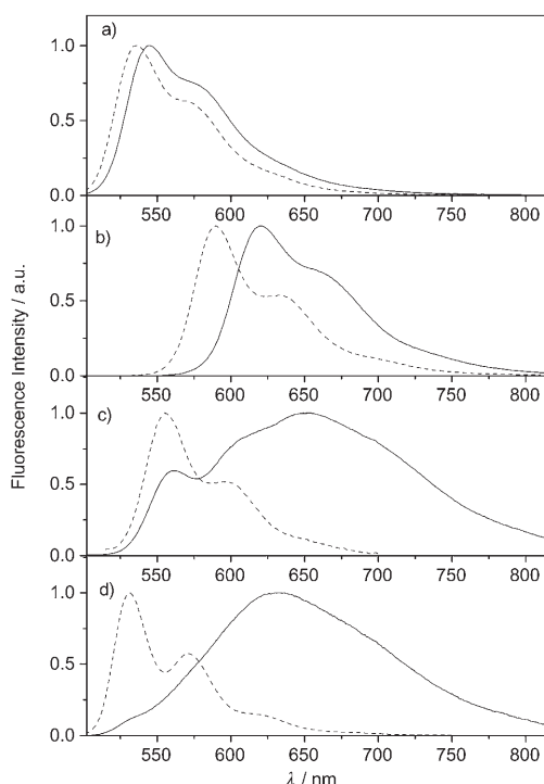
Figure 5. Normalized fluorescence spectra in MCH for a) 3a (at 1.0 \times 10^{-6} and 1.4 \times 10^{-2}\text{ M} ); b) 3b (at 1.0 \times 10^{-6} and 1.0 \times 10^{-2}\text{ M} ); c) 3e (at 2.0 \times 10^{-6} and 1.0 \times 10^{-3}\text{ M} ); and d) 3f (at 1.0 \times 10^{-6} and 1.0 \times 10^{-2}\text{ M} ). In all cases, a dashed line is used for the lower concentration and a solid line for the higher concentration.
