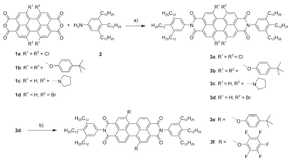
Scheme 1. Synthesis of PBIs 3a–f : a) \text{Zn}(\text{OAc})_2 , quinoline, 180^\circ\text{C} , 3 h, yields: 52 % ( 3a ), 53 % ( 3b ), 65 % ( 3c ), and 44 % ( 3d ); b) p - tert -butylphenol (for 3e ) or pentafluorophenol (for 3f ), \text{K}_2\text{CO}_3 , N -methyl-2-pyrrolidone (NMP), 120^\circ\text{C} , 2 h, yields: 40 % ( 3e ), and 61 % ( 3f ).
