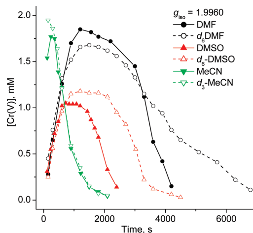
Figure 3. Typical kinetic curves for the formation of [\text{Cr}^{\text{V}}\text{O}(\text{SR})_4]^- ( g_{\text{iso}} = 1.9960 ) species in deuterated and undeuterated solvents during the reactions of [\text{Cr}^{\text{VI}}(\text{O})(\text{SR})_3]^- (10 mM) with RSH (250 mM) at 295 K, as observed by quantitative EPR spectroscopy with \text{Na}[\text{Cr}^{\text{V}}\text{O}(\text{ehba})_2] as an internal standard (see the Experimental Section for details). A full set of kinetic curves for all the reaction conditions listed in Table 2 is given in the kinetic curves for the reactions in mixed solvents (DMF/H 2 O or DMF/MeOH) shown in Figure S5, Supporting Information.
