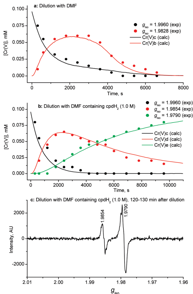
Figure 5. Typical kinetic curves (a, b) and EPR spectra (c) for the decomposition of [\text{Cr}^{\text{V}}\text{O}(\text{SR})_4]^- ( g_{\text{iso}} = 1.9960 species) in dilute DMF solutions at 295 K in the presence (b, c) or absence (a) of cis -1,2-cyclopentanediol (cpdH 2 , 1.0 M). The [\text{Cr}^{\text{V}}\text{O}(\text{SR})_4]^- complex was generated by the reaction of Cr(VI) (50 mM, from (\text{NH}_4)_2\text{Cr}_2\text{O}_7 ) with RSH (500 mM) in DMF for 15 min at 295 K, then the reaction mixture was diluted 100-fold with an appropriate solvent. Experimental kinetic data (dots in a and b) were obtained by quantitative EPR spectroscopy with \text{Na}[\text{Cr}^{\text{V}}\text{O}(\text{ehba})_2] as an internal concentration standard (see the Experimental Section). The EPR spectrum in c was obtained from an average of ten scans in the absence of the Cr(V) standard (the experimental conditions correspond to those in b, reaction time after the dilution 120–130 min). Calculated kinetic curves (lines in a and b) were obtained from the kinetic model in Table 2 (see text for details). Designations of the reaction intermediates (in italics) correspond to Table 2 and Scheme 1.
