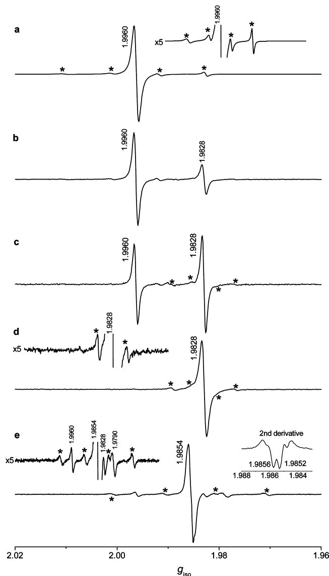
Figure 1. Typical EPR spectra (X-band, 295 K) of Cr(V) species formed during the reactions of Cr(VI) ( (\text{NH}_4)_2\text{Cr}_2\text{O}_7 , a–d) or Cr(V) ( \text{K}[\text{Cr}^{\text{VO}}(\text{cpd})_2] , where cpd = cis -1,2-cyclopentanediol, 16 (e) complexes with p -bromobenzenethiol (RSH) in DMF solutions. All the reactions were performed at 295 K, and the spectra were collected in the absence of a Cr(V) standard (see the Experimental Section). Signals due to the ^{53}\text{Cr} hyperfine splitting 8,12 are designated with asterisks. Reaction conditions: (a) Cr(VI) (50 mM) reacted with RSH (500 mM) in DMF for \sim 3 min, undiluted reaction mixture; (b) Cr(VI) (50 mM) reacted with RSH (500 mM) in DMF for 15 min, then the reaction mixture was diluted 100-fold with DMF, and the spectrum was collected at 5 min after the dilution; (c) same as (b), but 15 min after the dilution; (d) Cr(VI) (50 mM) reacted with RSH (500 mM) in DMF for 15 min, then the Cr(V) complexes were precipitated by a mixture of hexane and acetone (see the Experimental Section) and redissolved in DMF at [\text{Cr}] \sim 10 mM, the spectrum was recorded at \sim 3 min after the dissolution in DMF; and (e) Cr(V) (0.50 mM) reacted with RSH (10 mM) in DMF for \sim 3 min, undiluted reaction mixture.
