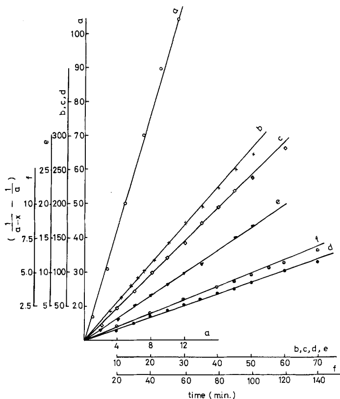
Fig. 1. Second order plots of 1/a-x-1/a against time for the reaction of 1 with different aromatic aldehydes: a Salicylaldehyde (20°C); b p -Dimethylaminobenzaldehyde (35°C); c p -Hydroxybenzaldehyde (35°C); d Vanilline (35°C); e Benzaldehyde (35°C); f p -Nitrobenzaldehyde (35°C)
