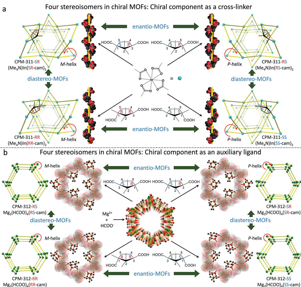
Figure 2. Chirality switching without topological change illustrated by two types of stereoisomerization in MOFs. a) In CPM-311, the crystallization between the monomeric \text{In}(\text{COO})_2 and four stereoisomers of camphoric acid leads to the same quartz type structure. b) In CPM-312, the crystallization between magnesium and formate form a honeycomb structure, with camphoric acid as a chiral pendant on the wall.
