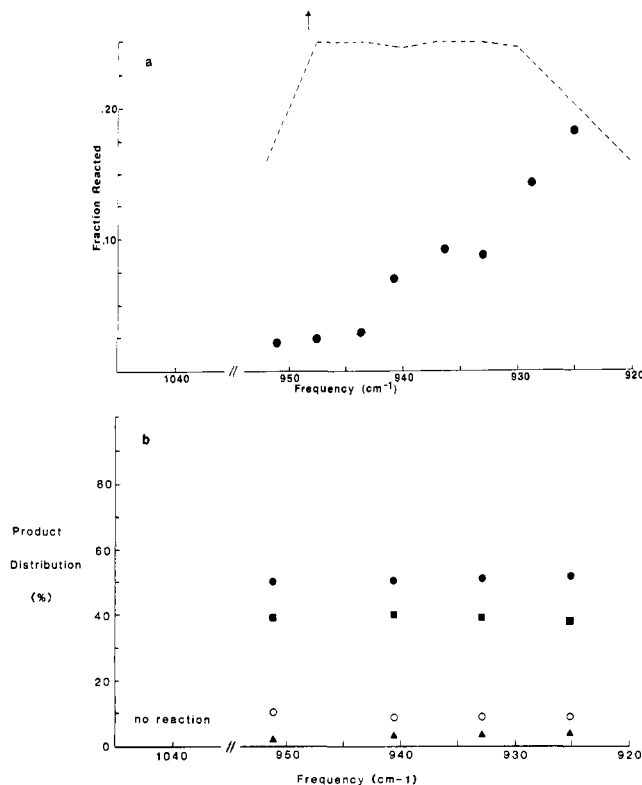
Figure 5. (a) Total product yield after 100 pulses vs. irradiation frequency. Dotted line represents relative absorbance for single photon absorption. Absorbance increases in the direction shown by the arrow. For standard conditions, see Table I. (b) Product ratio vs. irradiation frequency. Symbols are as those in Figure 2.
