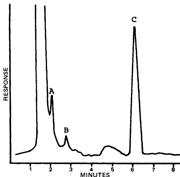
Figure 1—Typical gas chromatograph of a 1-ml human plasma extract spiked with 6 \mu g of clofibrate (A), 10 \mu g of clofibric acid (B), and 100 \mu g of benzocaine (C).
