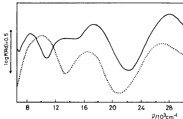
Fig. 2. Electronic spectra of \text{trans-[Ni(H}_2\text{O)}_2(\text{bezen})_2\text{Cl}_2] at room temperature (—) and at 110^\circ\text{C} (···).
