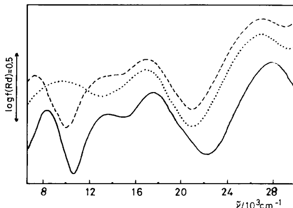
Fig. 3. Electronic spectra of \text{trans-[Ni(H}_2\text{O)}_2(\text{bezen})_2\text{Br}_2] at room temperature (—), at 120^\circ\text{C} (···) and at 150^\circ\text{C} (---).
