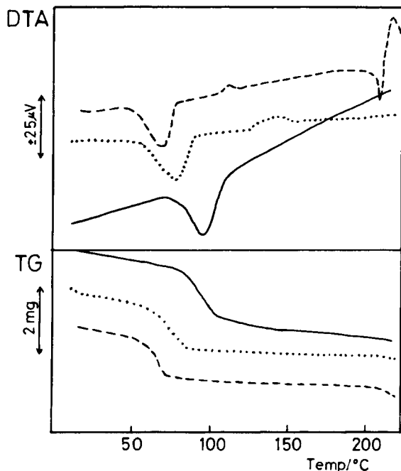
Fig. 1. TG-DTA results for \text{trans-[Ni(H}_2\text{O)}_2(\text{bezen})_2\text{X}_2\cdot n\text{H}_2\text{O]} , where X is \text{Cl}^- (—), \text{Br}^- (···) and \text{NO}_3^- (---), under a constant flow of \text{N}_2 at 0.2 \text{ dm}^3 \text{ min}^{-1} (heating rate, 2^\circ\text{C min}^{-1} for all runs; sample weight, 24.3, 26.0, and 19.9 mg for the chloride, bromide and nitrate, respectively).
