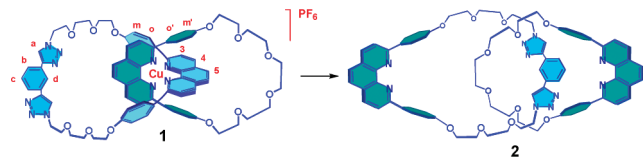
Figure 1. [2] catenane 1 and the corresponding [2] catenand 2 . After demetalation, a reorientation of the constituent rings results in a molecular conformation with the two phen ligands located away from each other.
