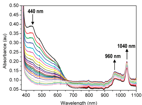
Figure 3. UV-vis kinetic study of the demetalation of catenate 1 in acetonitrile ( 10^{-5} mol L ^{-1} ) with \text{NH}_4\text{OH} ( 3 \times 10^{-4} mol L ^{-1} ), monitoring the absorbance at 440 nm. Total run time = 10 min, cycle time = 30 s, 298 K (au = arbitrary units).
