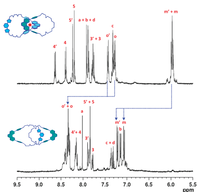
Figure 2. Partial ^1\text{H} NMR spectra of catenane 1 and the corresponding catenand 2 (400 MHz, \text{CD}_2\text{Cl}_2 , 298 K). For assignments, see Figure 1.
