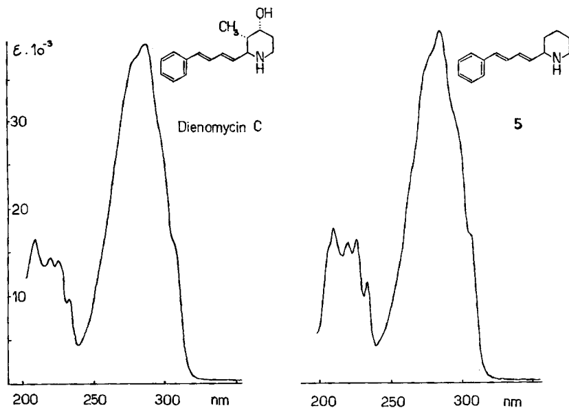
UV.-Spectrum in \text{CH}_3\text{OH} of Dienomycin-C-hydrochloride [7] and 5 -hydrochloride
