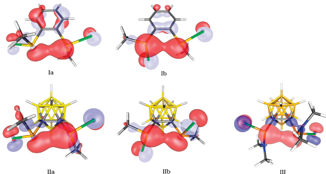
Figure 7. Geometrically optimized disubstituted compounds. P(Cl)(Me) derivatives occur in two conformations, denoted by a and b, respectively. Canonical molecular orbitals visualized with a spatial probability of 95%. The red and blue areas symbolize a positive or negative sign of the wave function, respectively. Ia (HOMO-1), Ib (HOMO-1), IIa (HOMO-2), IIb (HOMO-2), and III (HOMO-3); boron (tan), carbon (gray), chlorine (green), hydrogen (white), and phosphorus (orange).
