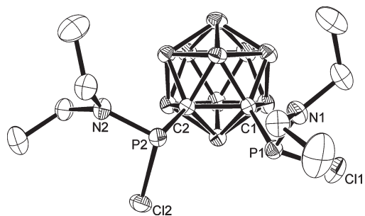
Figure 2. Molecular structure of 2b (ORTEP with atom labeling scheme; thermal ellipsoids are drawn at the 50% probability level; hydrogen atoms are omitted for clarity).
