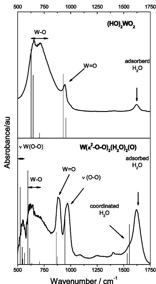
Figure 1. Experimental and theoretical IR spectra for tungstic acid and H 2 O 2 treated samples.
