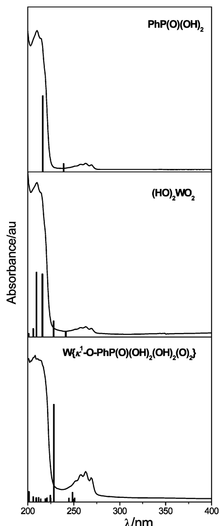
Figure 3. Experimental and theoretical UV-vis spectra of water diluted samples.
