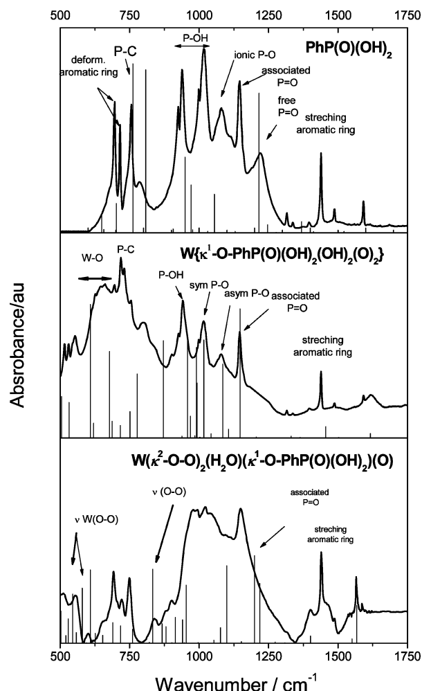
Figure 2. Experimental and theoretical IR spectra for phenylphosphonic acid, tungstic acid, and H 2 O 2 treated samples.
