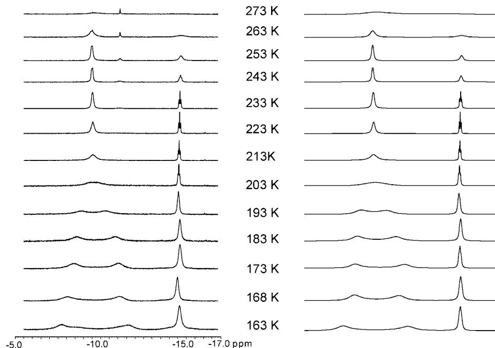
Figure 2. Variable-temperature ^1\text{H}\{^{31}\text{P}\} NMR spectra (400 MHz, \text{CDCl}_2\text{F} ) in the high-field region of [\text{OsH}(\eta^2\text{-H}_2)\{\kappa\text{C}^5, N\text{-}[1\text{-(2-pyridylmethyl)-3-methylimidazol-5-ylidene}]\}(\text{P}^i\text{Pr}_3)_2]\text{BPh}_4 ( 2a ): experimental (left); simulated (right).
