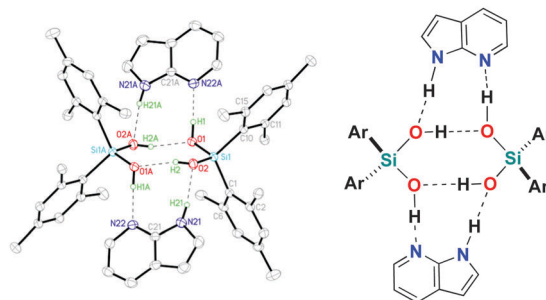
Fig. 3 Dimesitylsilane-1,2-diol (Ar = Mes) adduct with 7-azaindole (CCDC 958784). Thermal displacement plot shows 50% probability displacement ellipsoids for non-hydrogens. Selected hydrogens are omitted for clarity. Selected bond parameters [Å] for Mes 2 Si(OH) 2 :7-azaindole: H1...N22 1.79(3), O1...N22 2.6769(15), H2...O1A 1.91(2), O2...O1A 2.7049(14).
