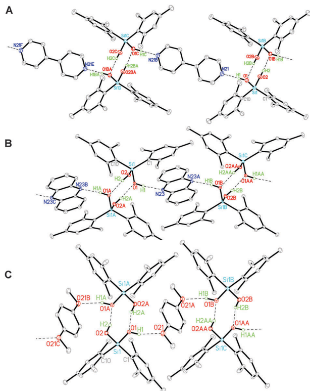
Fig. 2 Cyclic dimers of dimesitylsilane-1,2-diol are linked to form chains with 4,4'-bipyridine (A), phenazine (B), and 1,4-dimethoxybenzene (C). Thermal displacement plots show 50%, 30% and 30% probability displacement ellipsoids for non-hydrogens, respectively (CCDC 958825, 958790, 958824). Selected hydrogens and non-interacting CH 2 Cl 2 solvent molecules are omitted for clarity. Selected bond lengths [Å] for (A) Mes 2 Si(OH) 2 : 4,4'-bipy: H1...N21 1.88(2), O1...N21 2.7138(18); H2...O1B 2.00(2), O2...O1B 2.7476(16); (B) Mes 2 Si(OH) 2 :phenazine: H1...N23 1.946(19), O1...N23 2.7932(12); H2...O1A 1.920(19), O2...O1A 2.7446(11); (C) Mes 2 Si(OH) 2 :OMeAr: H1...O21 2.004(17), O1...O21 2.8399(9); H2...O1A 1.961(18), O2...O1A 2.8087(9). Distances between dimers (Å) = (A) 12.55, (B) 8.16, and (C) 9.14.
