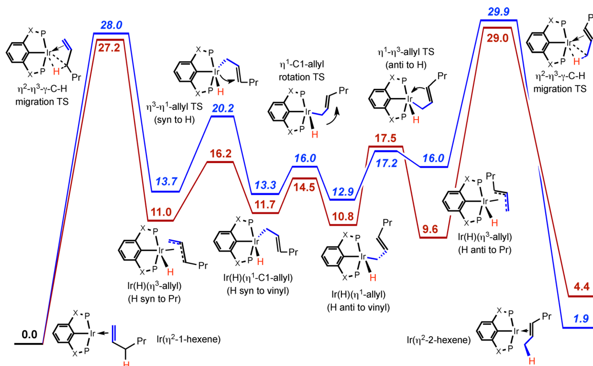
Figure 14. Pathway of \eta^2 - \eta^3 - \eta^1 ( \gamma -H migration) calculated for isomerization of bound 1-hexene/ trans -2-hexene, ( ^{t\text{Bu}}\text{POCOP} )Ir (X = O; blue, italicized free energy values) and ( ^{t\text{Bu}}\text{PCP} )Ir (X = CH 2 ; red).
