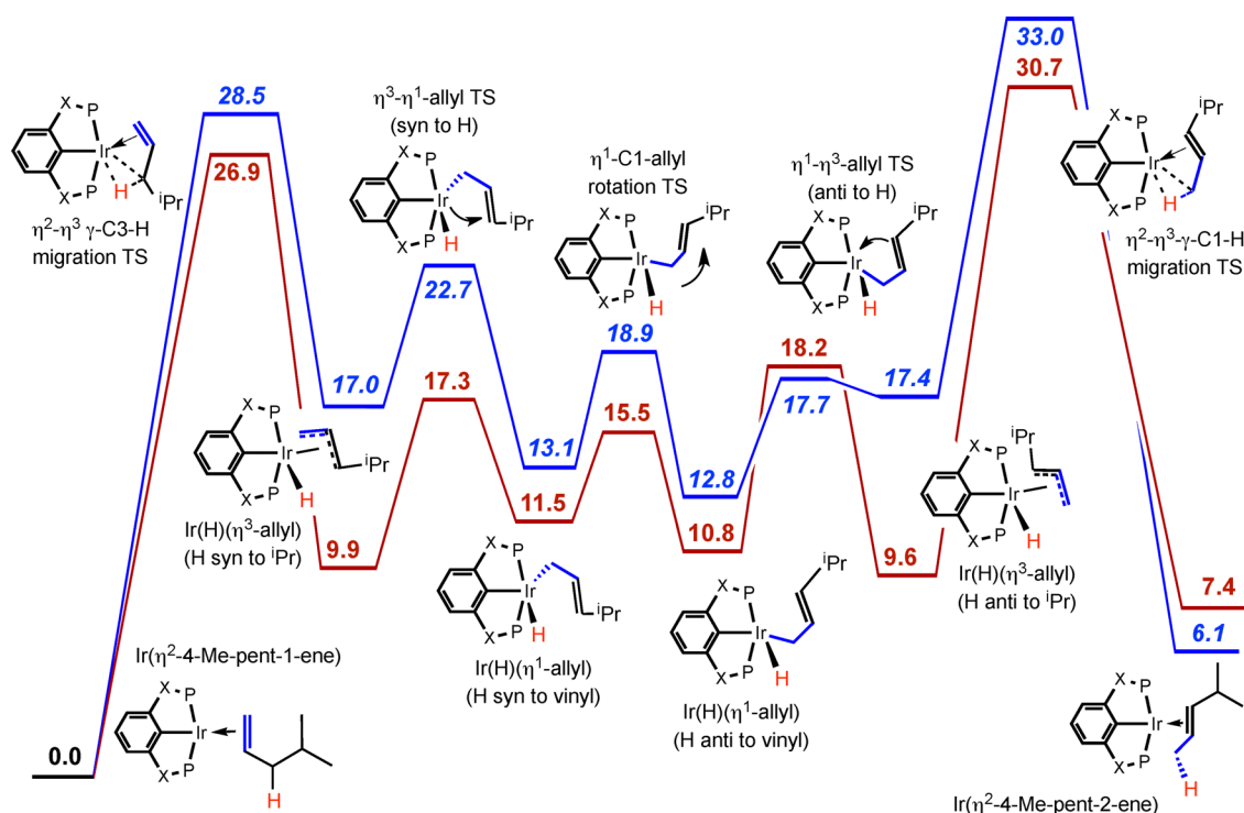
Figure 16. Calculated \eta^2 - \eta^3 - \eta^1 pathway for isomerization of bound 4-methylpent-1-ene/4-methylpent-2-ene, ( t\text{BuPOCOP} )Ir ( X = \text{O} ; blue, italicized free energy values) and ( t\text{BuPCP} )Ir ( X = \text{CH}_2 ; red).
