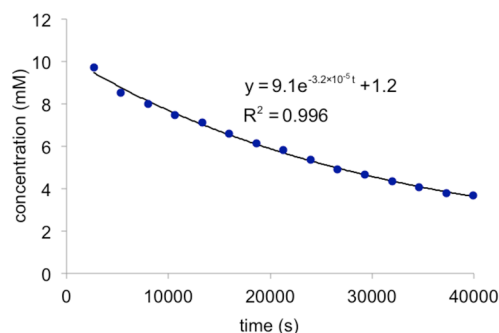
Figure 6. Isomerization of (t\text{BuPCP})\text{Ir}(\text{trans-2-hexene}) to (t\text{BuPCP})\text{Ir}(\text{1-hexene}) at 25 °C.
