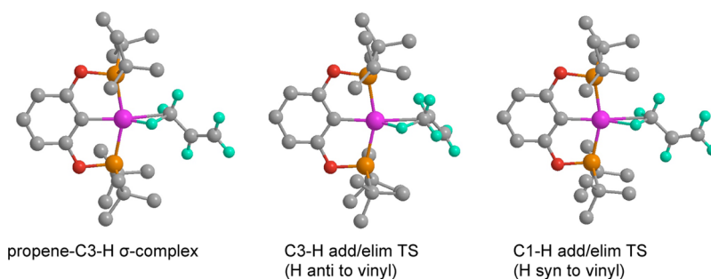
Figure 13. Molecular structures, unique to the \eta^2 - \eta^1 - \eta^3 pathway, of intermediates and transition states for double-bond migration in ( ^{t\text{Bu}}\text{POCOP} )Ir(propene) (for those species common to the \eta^2 - \eta^3 - \eta^1 pathway, see Figure 12). (O = red, P = orange, Ir = purple, C = gray, selected H atoms = blue; hydrogens on pincer ligand not shown.)
