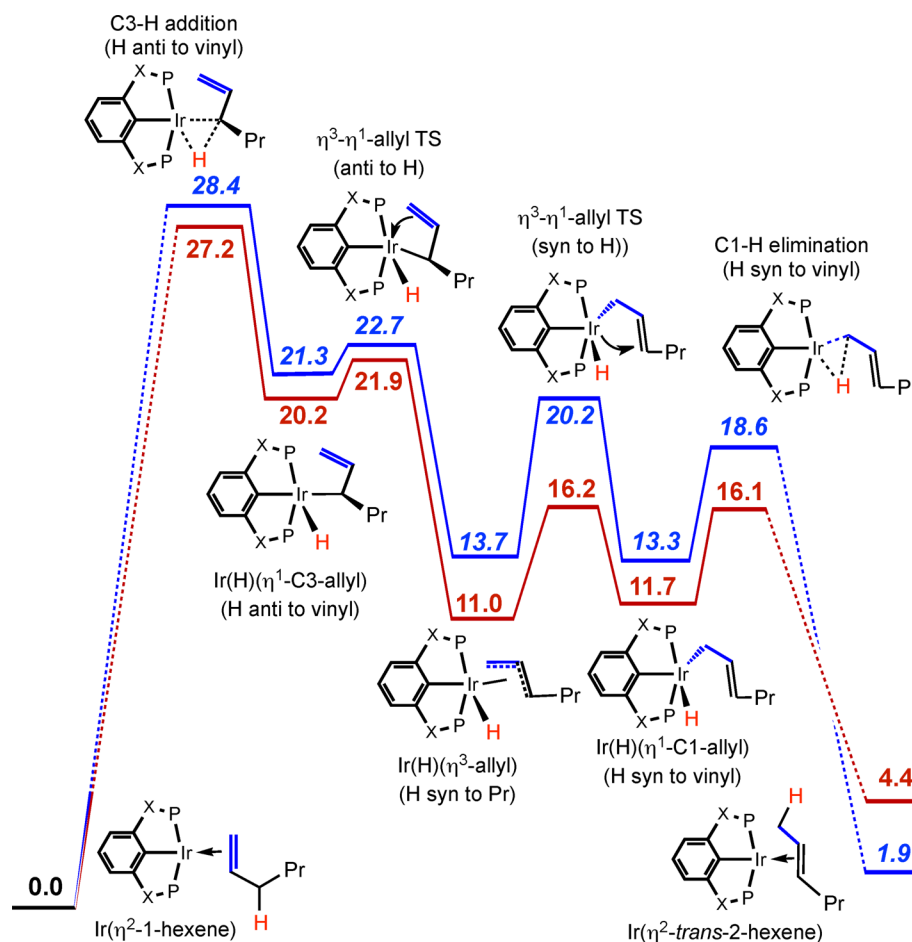
Figure 15. Pathway of \eta^2\text{-}\eta^1\text{-}\eta^3 (C–H addition) calculated for isomerization of bound 1-hexene/ trans -2-hexene, (t\text{BuPOCOP})\text{Ir} (X = O; blue, italicized free energy values) and (t\text{BuPCP})\text{Ir} (X = CH 2 ; red).
