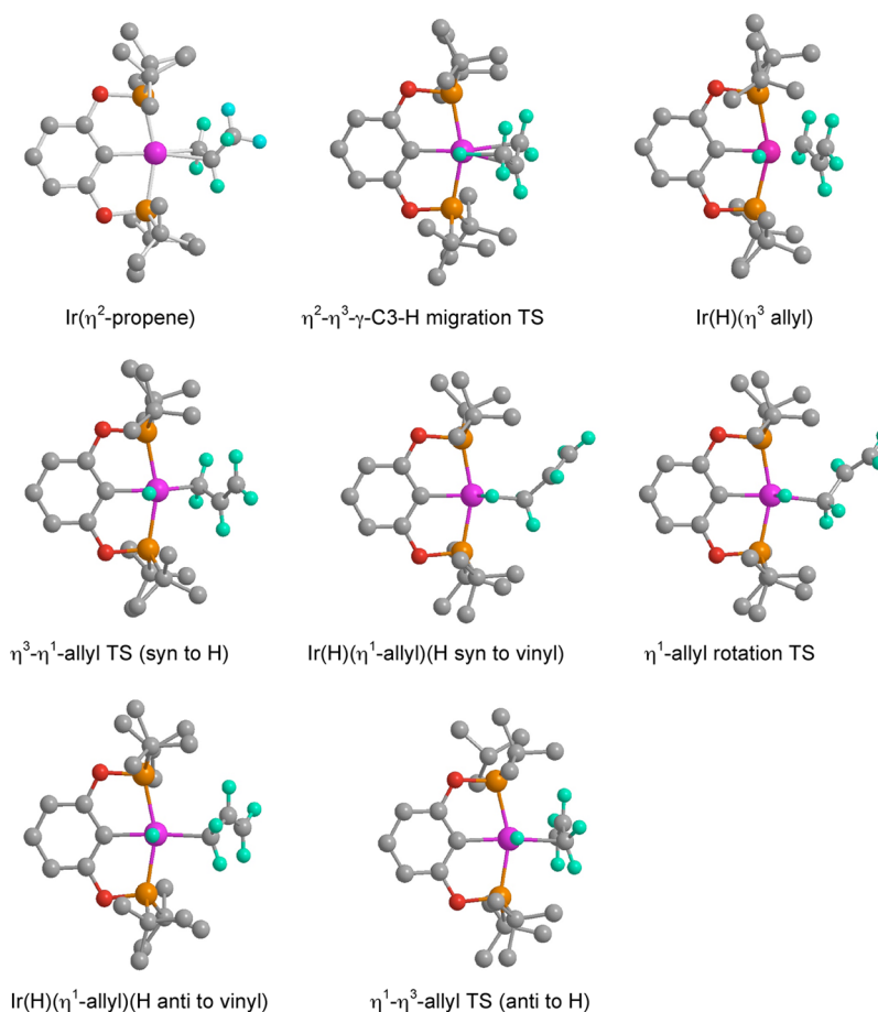
Figure 12. Molecular structures of intermediates and transition states for double-bond migration in ( t BuPOCOP)Ir(propene) via the \eta^2\text{-}\eta^3\text{-}\eta^1 pathway (O = red, P = orange, Ir = purple, C = gray, selected H = blue; hydrogens on pincer ligand not shown).
