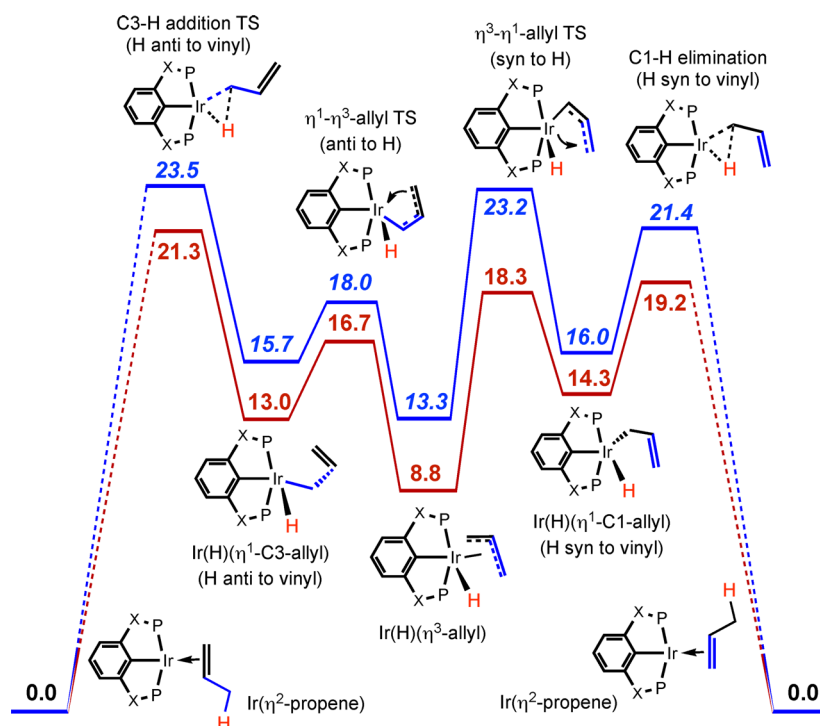
Figure 11. An \eta^2\text{-}\eta^1\text{-}\eta^3 pathway (C–H addition) calculated for 1,3-H migration of bound propene. ( t\text{BuPOCOP} )Ir (X = O; blue, italicized free energy values) and ( t\text{BuPCP} )Ir (X = \text{CH}_2 ; red). See Supporting Information for pathway connecting the C–H addition transition states with the propene complex.
