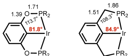
Scheme 10. Selected Distances (Å) and Angles in Calculated Structures of (^t\text{BuPCP})\text{Ir} and (^t\text{BuPOCOP})\text{Ir}
