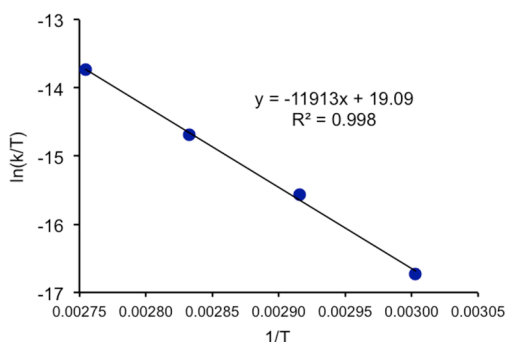
Figure 5. Eyring plot for the isomerization of (t\text{BuPOCOP})\text{Ir}(\text{trans-2-hexene}) to (t\text{BuPOCOP})\text{Ir}(\text{1-hexene}) in the temperature interval 60 to 90 °C.
