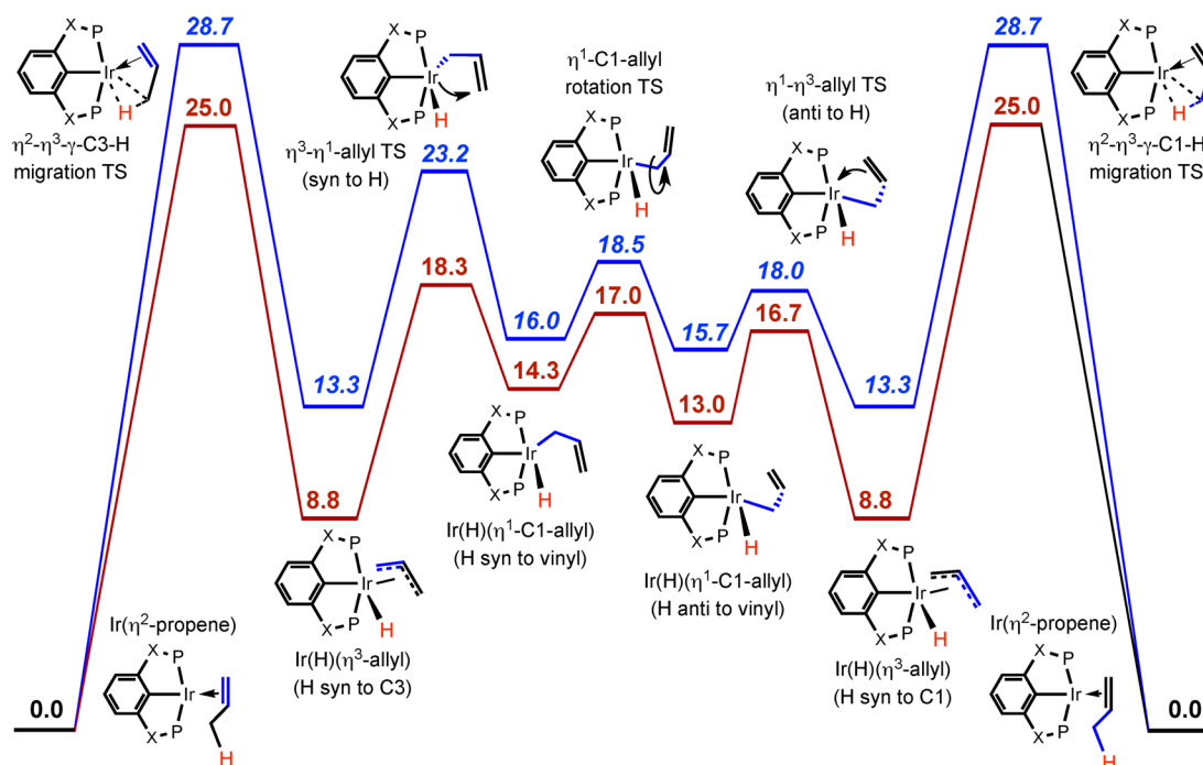
Figure 10. An \eta^2 - \eta^3 - \eta^1 rotation pathway ( \gamma -H migration) calculated for 1,3-H migration of bound propene, ( t\text{BuPOCOP} )Ir ( X = \text{O} ; blue, italicized free energy values) and ( t\text{BuPCP} )Ir ( X = \text{CH}_2 ; red).
