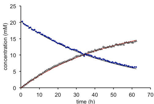
Figure 4. Isomerization of (t\text{BuPOCOP})\text{Ir}(\text{trans-2-hexene}) to (t\text{BuPOCOP})\text{Ir}(\text{1-hexene}) at 60 °C; curve shown represents a best fit to a first-order rate constant of 5.6 \times 10^{-6} \text{ s}^{-1} obtained using COPASI 31 kinetics fitting software.
