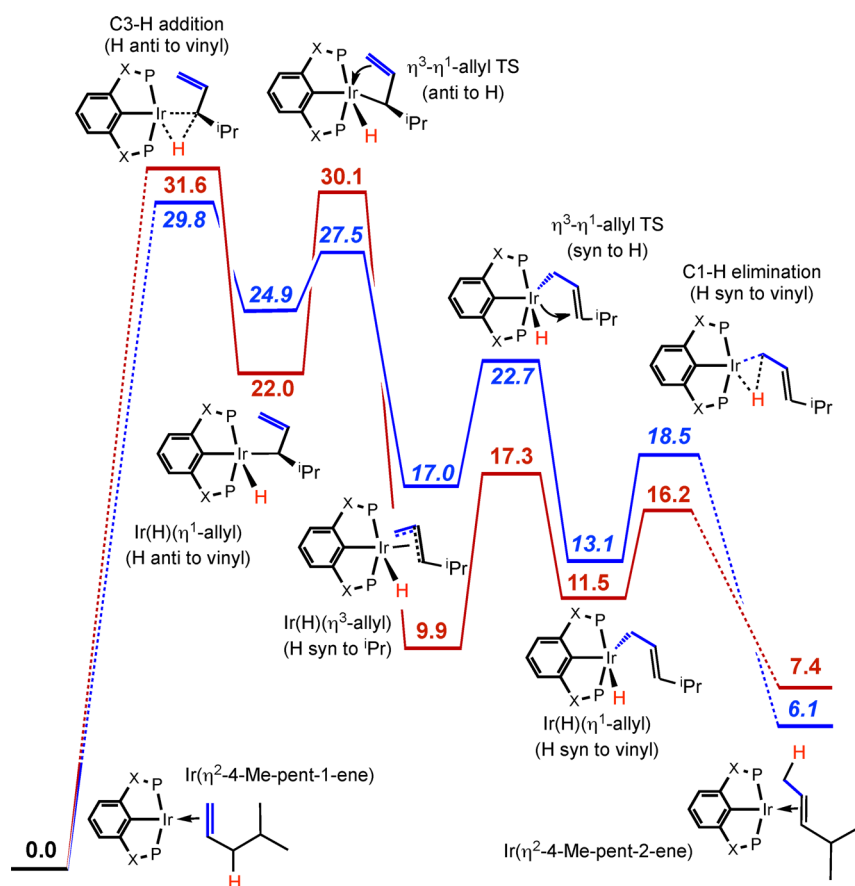
Figure 17. Calculated \eta^2 - \eta^1 - \eta^3 pathway for isomerization of bound 4-methylpent-1-ene/4-methylpent-2-ene, ( t\text{BuPOCOP} )Ir ( X = \text{O} ; blue, italicized free energy values) and ( t\text{BuPCP} )Ir ( X = \text{CH}_2 ; red).
