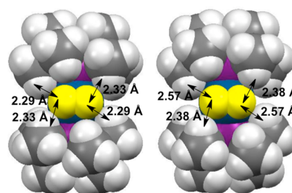
Scheme 12. Space-Filling Models of Calculated Structures of (^t\text{BuPCP})\text{IrH}_2 and (^t\text{BuPOCOP})\text{IrH}_2 (Ir-Bound Hydrides Yellow) with H( t Bu)-H(Hydride) Distances Indicated
