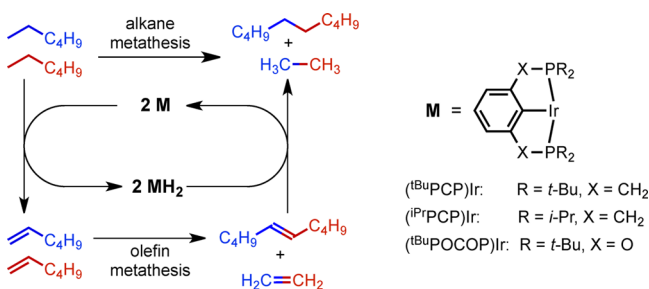
Scheme 2. Tandem Catalytic Alkane Metathesis with Pincer-Ligated Iridium Complexes and Olefin Metathesis Catalysts (Shown for Reaction of n -Hexane)
