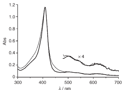
Figure 1. UV/Vis spectrum of m'-Hb (thin upper trace) compared with the spectrum of Hb (bold lower trace), both in 0.2 M phosphate buffer (pH 7.5) at 25 °C. The concentration of the proteins was 7.5 \mu\text{M} .
