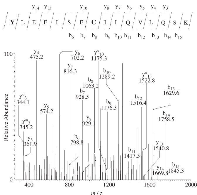
Figure 2. MS/MS spectrum of the m/z=995.5 peak (mass of 1989 amu) assigned to the 103–118 peptide in a double-charged state and with two modifications: the oxidation of C110 to the corresponding sulfinic acid, C110-SO 2 H, and the nitration of Y103 to 3-nitrotyrosine, Y103-NO 2 . The assignment of the y and b ion series is shown. Above the spectrum, the sequence of the 103–118 peptide, with the two modified amino acids in bold and with the summary of the y and b ions found in the spectrum, is reported.
