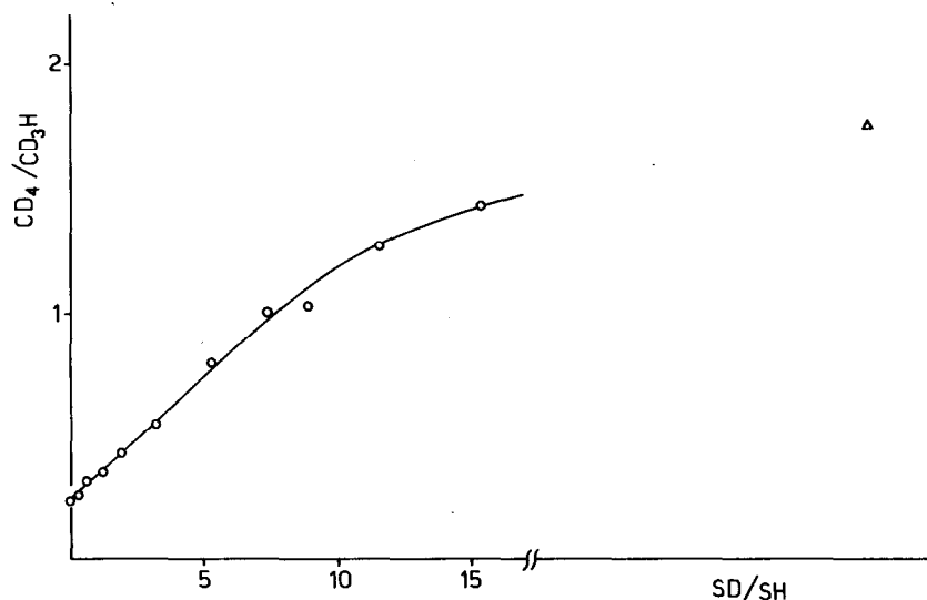
Fig. 1. The variation of \text{CD}_4/\text{CD}_3\text{H} with \text{SD}/\text{SH} for the thermolysis of \text{Pt}(\text{I})(\text{CD}_3)[\text{P}(\text{CH}_3)_3]_2 in \text{C}_6\text{D}_5\text{C}_2\text{D}_5 (SD)/ \text{C}_6\text{H}_5\text{C}_2\text{H}_5 (SH) mixtures at 120^\circ\text{C} ; \text{CD}_4/\text{CD}_3\text{H} in pure SD, \Delta .
