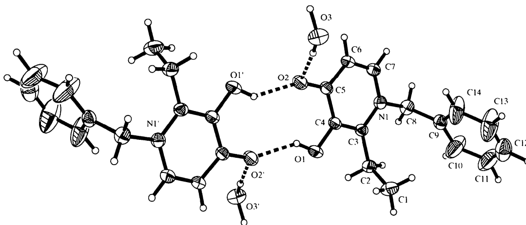
Fig. 1. The molecular structure of dimer (1) showing the atom-numbering scheme and 30% displacement ellipsoids. Primed atoms are generated by a centre of symmetry [symmetry code: ( ' ) -x, -y, -z ]. Intermolecular O—H...O bonds are shown as dashed lines. H atoms are drawn as spheres of arbitrary radii.
