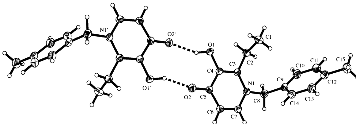
Fig. 2. The molecular structure of (2) showing the atom-numbering scheme and 30% displacement ellipsoids. Primed atoms are generated by a centre of symmetry [symmetry code: ( ' ) 1-x, 1-y, -z ]. Intermolecular hydrogen bonds are shown as dashed lines.
