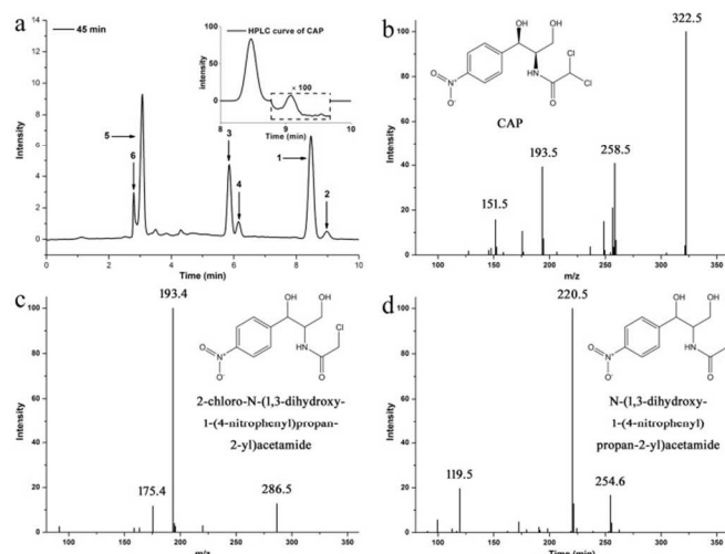
Figure 4. HPLC and LC-MS of CAP and its by-products (a) HPLC spectrum of CAP treated with 717@Au-Pd for 45 min, (b) LC-MS of CAP, (c) LC-MS of 2-chloro-N-(1,3-dihydroxy-1-(4-nitrophenyl)propan-2-yl)acetamide, (d) LC-MS of N-(1,3-dihydroxy-1-(4-nitrophenyl)propan-2-yl)acetamide.
