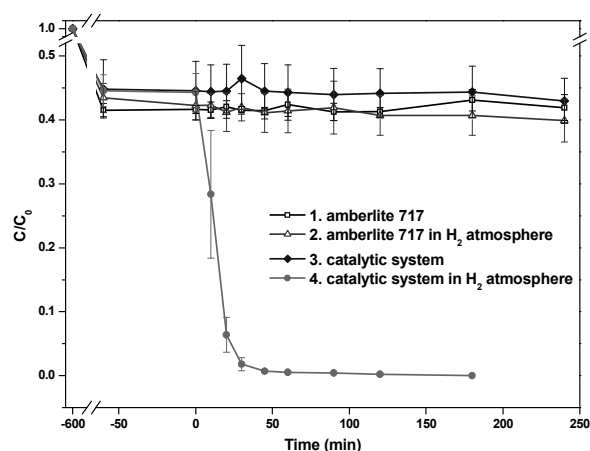
Figure 3. Concentration variation of CAP with different experimental conditions, C 0 : 50 mg L -1 .
