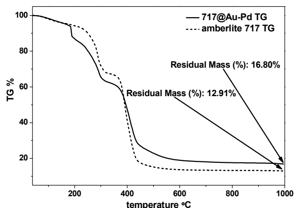
Figure 2. TG and DTG curves of amberlite 717 and 717@Au-Pd.
