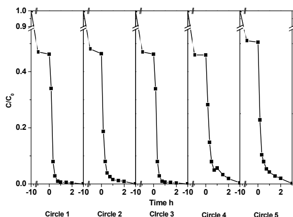
Figure 6. Cycling tests of degradation reaction of CAP by using 717@Au-Pd as catalysts, C_0 : 50 mg L -1 .
