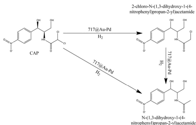
Figure 5. The reaction route of CAP in H 2 environment with 717@Au-Pd.
