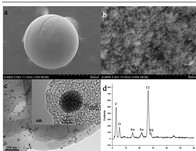
Figure 1. SEM images of 717@Au-Pd of low magnification (a), high magnification (b), HRTEM image of 717@Au-Pd (c) and EDAX spectra of 717@Au-Pd (d).
