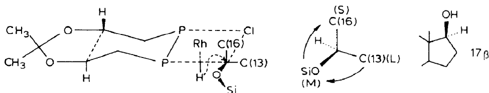
Fig. 3. Interaction of (+)( R,R )-DIOP with incipient formation of 17β-estradiol.
