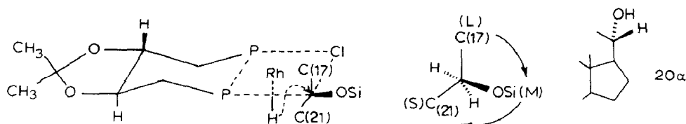
Fig. 8. Interaction of (+)( R,R )-DIOP with incipient formation of 20 \alpha -hydroxy-pregna-3,5-diene.
