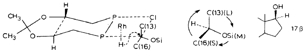
Fig. 4. Interaction of (+)( R,R )-DIOP with incipient formation of 17β-estradiol.
