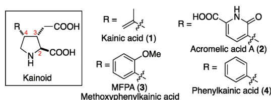
Figure 1. Structures of kainoids 1, 2, 3, and 4.
