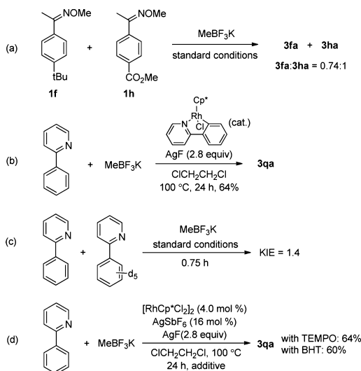
Scheme 4. Mechanistic Studies
