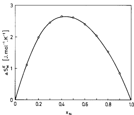
FIG. 4. Excess integral entropy of mixing at 1400K.
