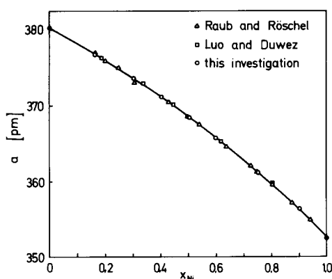
FIG. 1. Lattice constants of the system rhodium-nickel.
