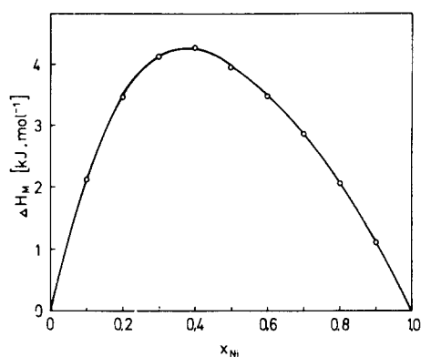
FIG. 5. Integral enthalpy of mixing of rhodium-nickel alloys at 1400K.
