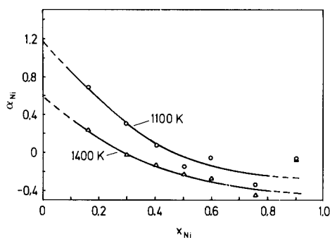
FIG. 3. \alpha function for nickel in rhodium-nickel alloys.
