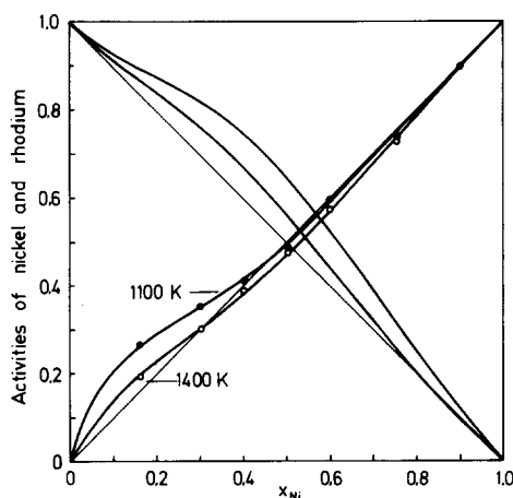
FIG. 2. Activities of nickel and rhodium at 1100 and 1400K.
