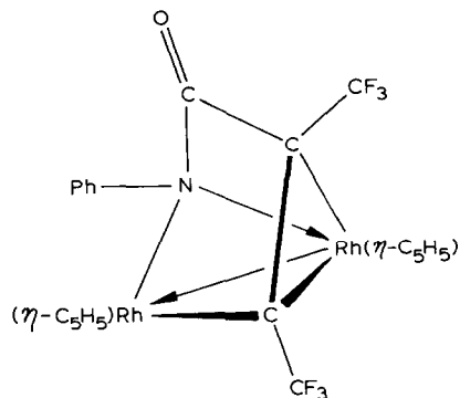
Fig. 2. Coordination mode of the bridging ligand in the complex (\eta\text{-C}_5\text{H}_5)_2\text{Rh}_2[\mu_2(\eta^3\text{-C(CF}_3\text{)}_2\text{C(CF}_3\text{)C(O)N(R)})] .
