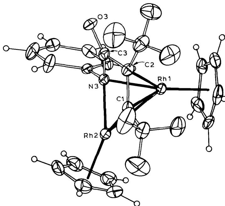
Fig. 1. Molecular structure of (\eta\text{-C}_5\text{H}_5)_2\text{Rh}_2[\mu_2(\eta^3\text{-C(CF}_3\text{)}_2\text{C(CF}_3\text{)C(O)N(Ph)})] . Bond lengths: Rh(1)–Rh(2) 2.612(1), Rh(1)–C(1) 2.020(9), Rh(2)–C(1) 2.148(8), Rh(1)–C(2) 2.138(8), Rh(1)–N(3) 2.169(6), Rh(2)–N(3) 2.049(6), C(1)–C(2) 1.45(1), C(2)–C(3) 1.48(1), C(3)–O(3) 1.20(1), C(3)–N(3) 1.41(1) Å.
