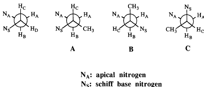
Fig. 2. Staggered conformation of the N_A -CH 2 -CH 2 -N S fragments found in the X-ray structures [ML^2] ( M =Fe, Cr, Mn) (left) and possible eclipsed conformations A, B, and C of the N_A -CH 2 -CH(CH 3 )-N S fragments of ligands [H_3L^5] and [H_3L^6] ( N_A : apical nitrogen, N_S : Schiff base nitrogen)
