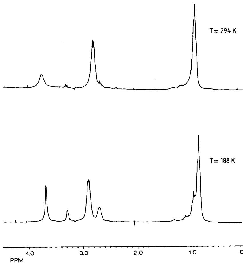
Fig. 1. 1 H NMR spectra of a mixture of RhCl(CO)(ddpa) 2 and ddpa in CD 2 Cl 2 at selected temperatures.
