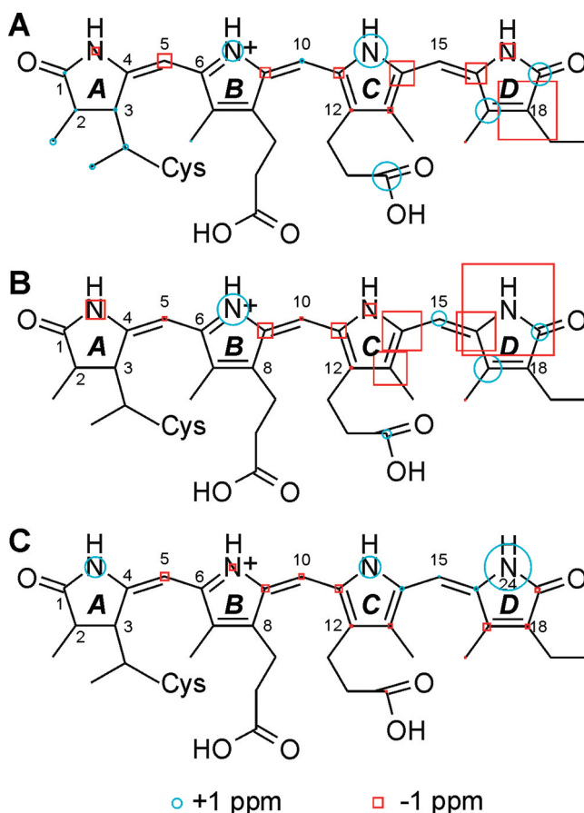
Figure 3. Changes in ^{13}\text{C} and ^{15}\text{N} chemical shift of the u- ^{13}\text{C} , ^{15}\text{N} -PCB chromophore in Cph1Δ2 during the Pfr → Lumi-F (A), Lumi-F → Meta-F (B), and Meta-F → Pr (C) transitions. For each transition, the starting state is taken as reference and the size of the circles and squares refers to the difference in ^{13}\text{C} and ^{15}\text{N} chemical shift in the next state.
