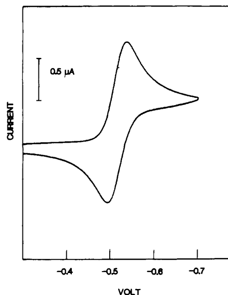
Figure 3. Cyclic voltammogram of [(\eta^5-C_5(CH_3)_5)Ir(\eta^6-C_6(CH_3)_6)]^{2+} ( 2b^{2+} ) 0.10 mM in CH_2Cl_2/0.1 M TBAHFP at a hanging mercury drop electrode ( \nu = 0.1 V/s).
