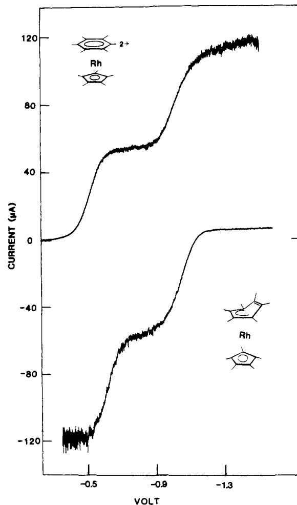
Figure 2. Voltammograms at a rotating platinum electrode in CH_2Cl_2/0.1 M TBAHFP: (top) initial, 1.5 mM 2a 2+ ; (bottom) after electrolysis at -1.3 V to 95% depletion of electrolysis current at a platinum basket electrode to pass 1.93 F.
