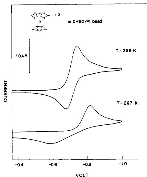
Figure 4. Cyclic voltammogram of [(\eta^5-C_5(CH_3)_5)Ir(\eta^6-C_6(CH_3)_6)]^{2+} ( 2b^{2+} ) 0.38 mM in Me_2SO/0.1 M TBAHFP at a platinum bead electrode ( \nu = 0.13 V/s, temperature 358 (top) and 297 K (bottom)).
