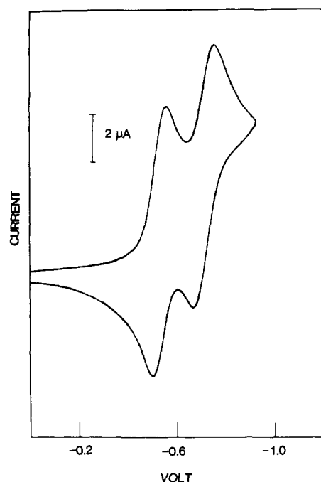
Figure 1. Cyclic voltammogram of [\eta^5\text{-C}_5(\text{CH}_3)_5]\text{Rh}[\eta^6\text{-C}_6(\text{CH}_3)_6]^{2+} ( 2a^{2+} 0.42 mM in acetone/0.1 M TBAHFP at a platinum bead electrode ( \nu = 0.1 \text{ V/s} ).
