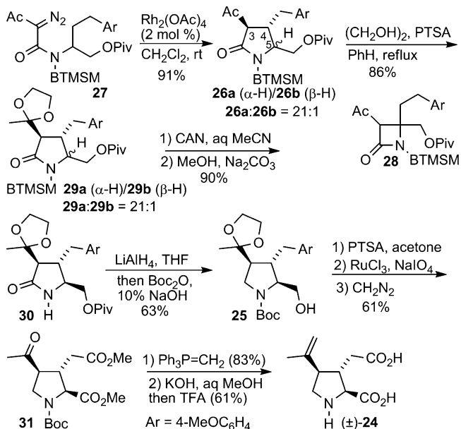
Scheme 1. Synthesis of 24
