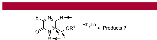
Figure 1. Potential C–H insertion sites.
