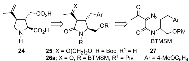
Figure 2. Retrosynthesis of 24 .
