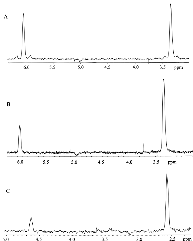
Figure 2. Magnetization transfer difference spectra: (A) complex 1 at 80 °C: selective irradiation at \delta 3.33 ppm; (B) complex 1 at 60 °C: selective irradiation at \delta 3.33 ppm; (C) complex 2 at 20 °C: selective irradiation at \delta 2.66 ppm.
