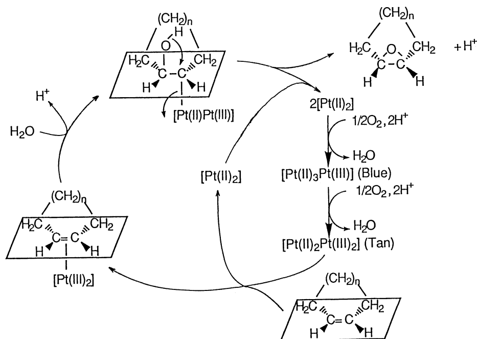
Fig. 1. Possible mechanism for the epoxidation reaction.
