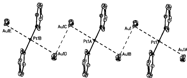
Figure 6. View of the extended structure of [\text{Pt}(\text{bipy})_2][\text{Au}(\text{CN})_2]_2 with 50% thermal contours including the interactions of adjacent anions. The \text{Au1}\cdots\text{Au1B} distance is 3.5978(9) Å.
