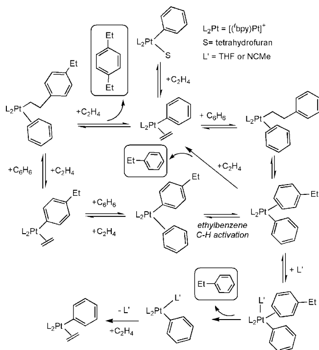
Scheme 1. Possible Catalytic Cycle To Produce Ethylbenzene and Diethylbenzene from Benzene and Ethylene Catalyzed by 3 a
