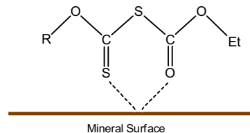
Scheme 2. Schematic representation of the potential chelating ability of the SS conformer of ROC(S)SC(O)OEt molecules during a flotation process.
