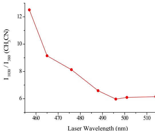
Fig. 6. Raman excitation profile of the 1030 \text{ cm}^{-1} band assigned to \nu(\text{C}=\text{S}) of \text{CH}_3(\text{CH}_2)_2\text{OC}(\text{S})\text{SC}(\text{O})\text{OCH}_2\text{CH}_3 with respect to the 380 \text{ cm}^{-1} band of \text{CH}_3\text{CN} .
