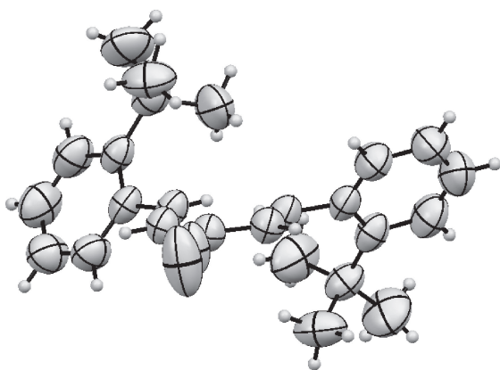
Figure 2. X-ray crystallographic chart of 1e .
