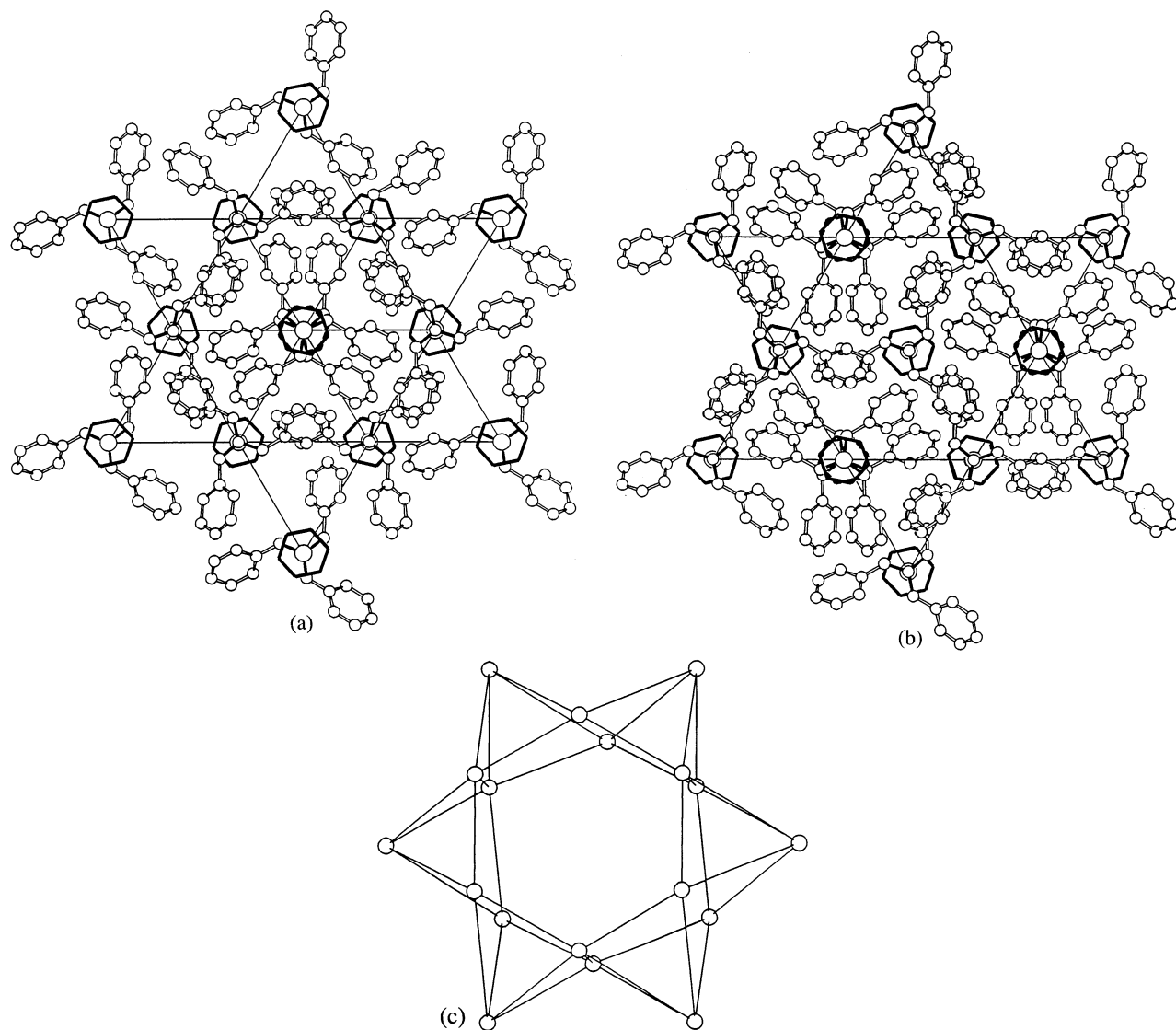
Fig. 5. (a) Crystal packing of 1a . SCHAKAL view parallel to the trigonal axis, showing the coordination of the molecule on (0\ 0\ z) . (b) Crystal packing of 1a . SCHAKAL view parallel to the trigonal axis, showing the coordination of the molecule on (2/3\ 1/3\ z) . (c) Same as (b), showing only the metal atom positions of the coordinating molecules. The view is slightly tilted from the trigonal axis.
