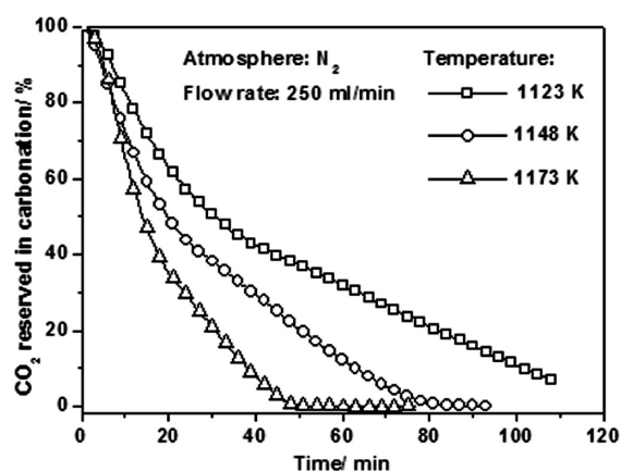
Figure 9. Kinetics of CO 2 desorption from the absorbed Li 8 ZrO 6 at different temperatures in a N 2 atmosphere with a flow rate of 250 mL min -1 .
