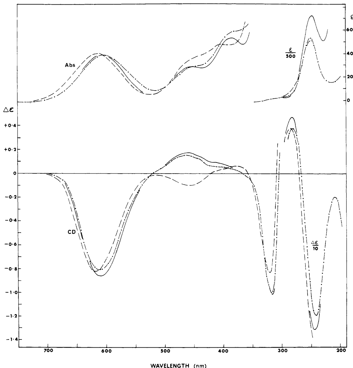
Figure 4. UV-visible absorption and circular dichroism spectra of trans -[CoCl 2 (( S )-dmbn) 2 ] + in acetonitrile (—) as the tetraphenylborate salt and in methanol (---) and dimethyl sulfoxide (-.-) as the perchlorate salt.
