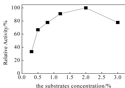
Fig. 8. Optimum Concentration of Substrate of Dioscin- \alpha -L-rhamnosidase
