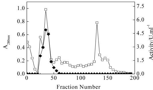
Fig. 2. DEAE-Cellulose Chromatography of Dioscin- \alpha -L-rhamnosidase Column, DEAE-cellulose column (2 \times 15 cm); solvent, 0–0.6 M KCl in 20 mM pH 7.2 Tris–HCl buffer; fraction, 3 ml; eluting rate, 3 ml/min; \square , protein; \blacklozenge , enzyme activity.
