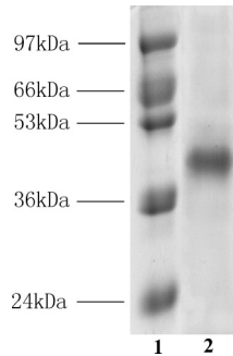
Fig. 3. SDS–Polyacrylamide Gel Electrophoresis of Dioscin- \alpha -L-rhamnosidase 1: standard proteins; 2: dioscin- \alpha -L-rhamnosidase; standard proteins: trypsinogen (24 kDa), glyceraldehyde-3-phosphate-dehydrogenase (36 kDa), glutamic dehydrogenase (53 kDa), albumin (66 kDa), phosphorylase (97 kDa).
