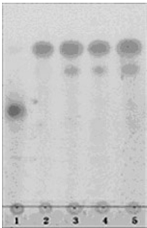
Fig. 4. TLC of Dioscin Hydrolysis by Enzyme The reaction mixture containing 0.1 ml of the substrate and 0.1 ml of the enzyme was incubated for 24 h at 37 °C. The reaction was stopped by the addition of 0.2 ml of n -butanol saturated water. An aliquot of the n -butanol layer was applied on TLC: solvent, chloroform–methanol–water (70 : 30 : 5, v/v/v); detection, 10 % sulfuric acid. 1: standard dioscin; 2: standard diosgenyl- O - \beta -D-Glc; 3, 4, and 5, three products from the enzyme reaction.
