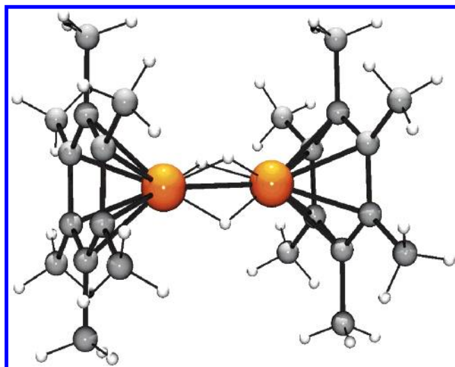
Figure 2. Molecular structure of [(\eta^6\text{-C}_6\text{Me}_6)_2\text{Ru}_2(\mu_2\text{-H})_3]^+ .
