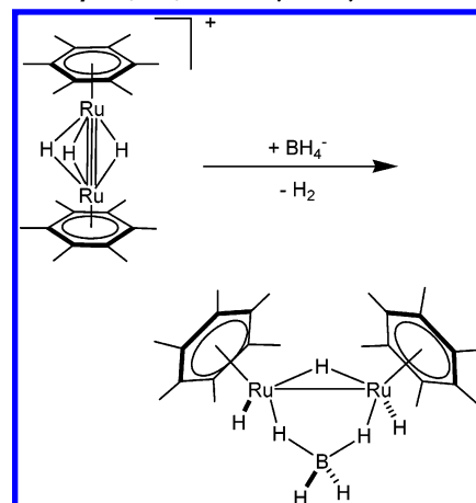
Scheme 3. Reaction of [(\eta^6\text{-C}_6\text{Me}_6)_2\text{Ru}_2(\mu_2\text{-H})_3]^+ with Sodium Borohydride in Water To Give [(\eta^6\text{-C}_6\text{Me}_6)_2\text{Ru}_2\text{H}_2(\mu_2\text{-H})(\mu_2\text{-BH}_4)]
