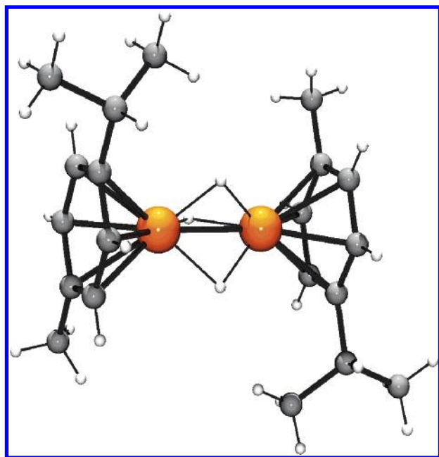
Figure 1. Molecular structure of [(\eta^6\text{-}1,4\text{-}i\text{PrC}_6\text{H}_4\text{Me})_2\text{Os}_2(\mu_2\text{-H})_3]^+ .
