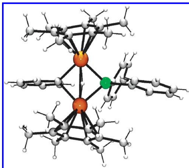
Figure 3. Molecular structure of the cation [(\eta^6\text{-C}_6\text{Me}_6)_2\text{Ru}_2(\mu_2\text{-PPH}_2)(\mu_2\text{-H})(\mu_2\text{-Ph})]^+ .
