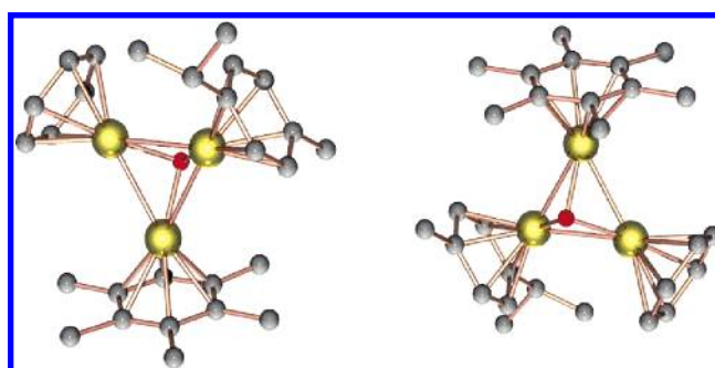
Figure 4. The two enantiomers ( S )- and ( R )- [(\eta^6\text{-C}_6\text{H}_6)(\eta^6\text{-C}_6\text{Me}_6)(\eta^6\text{-1,4-}^i\text{PrC}_6\text{H}_4\text{Me})\text{Ru}_3(\mu_2\text{-H})_3(\mu_3\text{-O})]^+ , present in the crystal of the hexafluorophosphate salt.
