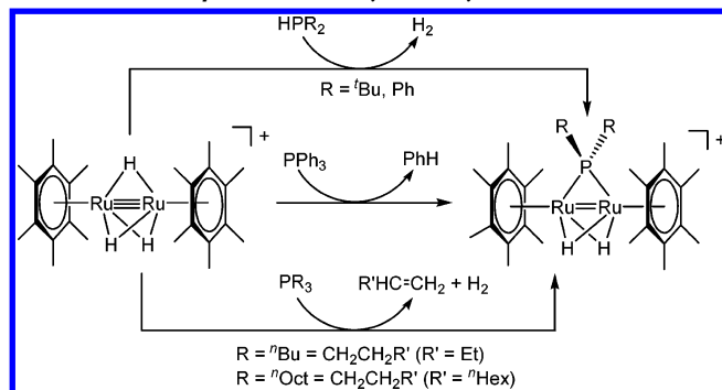
Scheme 7. Reaction of [(\eta^6\text{-C}_6\text{Me}_6)_2\text{Ru}_2(\mu_2\text{-H})_3]^+ with Secondary and Tertiary Phosphines to Give the Monophosphido Derivatives [(\eta^6\text{-C}_6\text{Me}_6)_2\text{Ru}_2(\mu_2\text{-PR}_2)(\mu_2\text{-H})_2]^+
