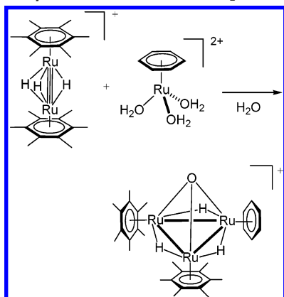
Scheme 9. Synthesis of the Trinuclear Cluster [(\eta^6\text{-C}_6\text{H}_6)(\eta^6\text{-C}_6\text{Me}_6)_2\text{Ru}_3(\mu_2\text{-H})_3(\mu_3\text{-O})]^+ from the Dinuclear Precursor [(\eta^6\text{-C}_6\text{Me}_6)_2\text{Ru}_2(\mu_2\text{-H})_3]^+ and the Mononuclear Complex [(\eta^6\text{-C}_6\text{H}_6)\text{Ru}(\text{H}_2\text{O})_3]^{2+} in Aqueous Solution
