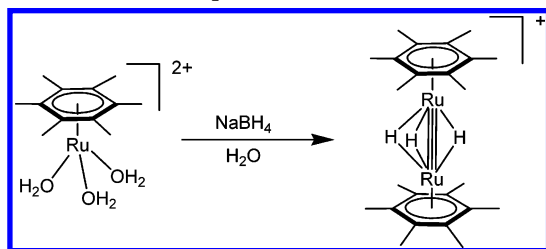
Scheme 1. High-Yield Synthesis of [(\eta^6\text{-C}_6\text{Me}_6)_2\text{Ru}_2(\mu_2\text{-H})_3]^+ from the Aquo Complex [(\eta^6\text{-C}_6\text{Me}_6)_2\text{Ru}(\text{OH}_2)_3]^{2+} and Sodium Borohydride in O 2 -Free Aqueous Solution
