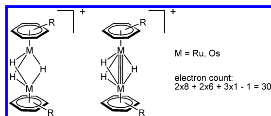
Chart 1. Alternative Representations of the Electron-Deficient Complexes [( \eta^6 -arene) 2 M 2 ( \mu_2 -H) 3 ] + with Three Three-Center Bonds or with a Metal–Metal Triple Bond
