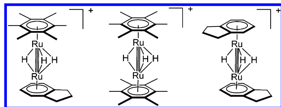
Chart 2. The Three Mixed (One Asymmetrical and the Two Symmetrical) Diruthenium Trihydrido Cations Formed by Reaction of NaBH 4 with a Mixture of [(\eta^6\text{-C}_6\text{Me}_6)\text{Ru}(\text{OH}_2)_3]^{2+} and [(\eta^6\text{-C}_9\text{H}_9)\text{Ru}(\text{OH}_2)_3]^{2+} in Aqueous Solution
