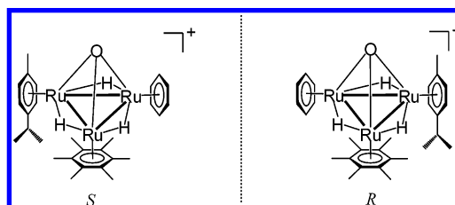
Chart 4. S and R Enantiomers of the Intrinsically Chiral Cluster Cation [(\eta^6\text{-C}_6\text{H}_6)(\eta^6\text{-C}_6\text{Me}_6)(\eta^6\text{-1,4-}^i\text{PrC}_6\text{H}_4\text{Me})\text{Ru}_3(\mu_2\text{-H})_3(\mu_3\text{-O})]^+ , Containing a Tetrahedral \text{Ru}_3\text{O} Skeleton with Four Different Vertices
