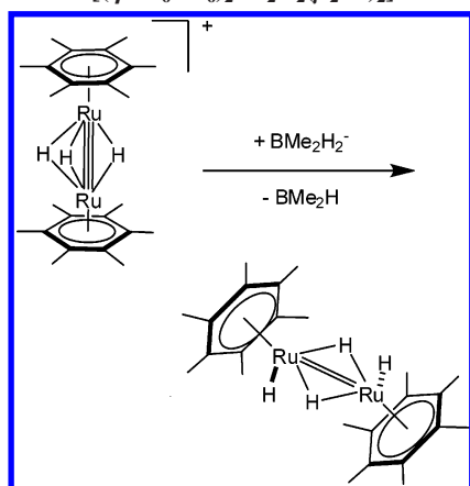
Scheme 2. Reaction of [(\eta^6\text{-C}_6\text{Me}_6)_2\text{Ru}_2(\mu_2\text{-H})_3]^+ with Lithium Dimethylborate in Hexane–Water To Give [(\eta^6\text{-C}_6\text{Me}_6)_2\text{Ru}_2\text{H}_2(\mu_2\text{-H})_2]
