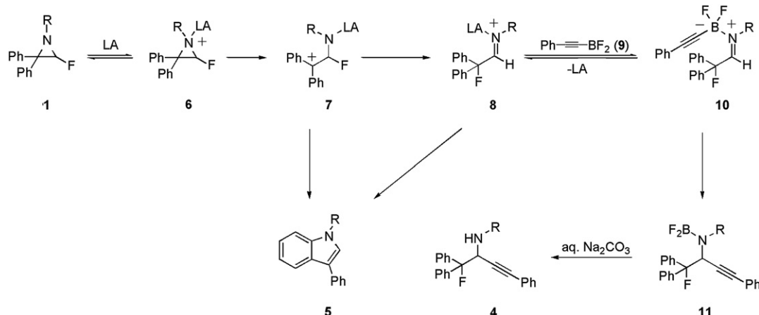
Scheme 2. Reaction mechanism.
