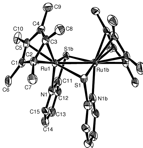
Figure 1. ORTEP drawing (50% thermal ellipsoids) of [\{\text{Cp}^*\text{Ru}(\text{SC}_5\text{H}_4\text{N})\}_2]^{2+} in 7 . Hydrogen atoms have been omitted. Selected bond lengths ( \text{\AA} ) and angles ( ^\circ ) with estimated standard deviations in parentheses: \text{Ru1--Ru1b} 2.4964(10) , \text{Ru1--S1} 2.4218(13) , \text{Ru1--S1b} 2.4512(12) , \text{Ru1--N1} 2.163(4) ; \text{Ru1--S1--Ru1b} 61.63(4) , \text{S1--Ru1--S1b} 117.18(4) , \text{N1--Ru1--S1b} 66.52(11) .
