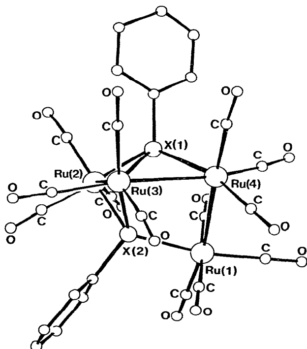
Fig. 1. The molecular stereochemistry of [\text{Ru}_4(\mu_3\text{-XPh})_2(\text{CO})_{13}] (X = P or As). Some relevant bond lengths in Å. IIIa (X = P): Ru(1)—Ru(4), 2.903(1); Ru(2)—Ru(3), 2.885(1); Ru(3)—Ru(4), 2.926(1); Ru(1)—P(2), 2.420(1); Ru(2)—P(1), 2.335(1); Ru(2)—P(2), 2.372(1); Ru(3)—P(1), 2.395(1); Ru(3)—P(2), 2.374(1); Ru(4)—P(1), 2.343(1); IIIb (X = As): Ru(1)—Ru(4), 2.928(9); Ru(2)—Ru(3), 2.927(8); Ru(3)—Ru(4), 2.969(8); Ru(1)—As(2), 2.504(8); Ru(2)—As(1), 2.422(8); Ru(2)—As(2), 2.475(7); Ru(3)—As(1), 2.508(8); Ru(3)—As(2), 2.472(8); Ru(4)—As(1), 2.437(8).
