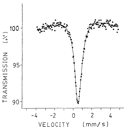
Fig. 1. Mössbauer spectrum of tetrachloro-1,4-di[ p -methoxyphenyl]-2,3-dimethyl-1,4-diazabutadiene]-tin(IV) at 77°K
