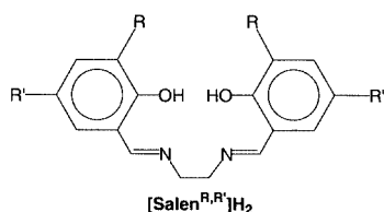
Fig. 1 The [\text{Salen}^{\text{R}, \text{R}'}]\text{H}_2 system.
