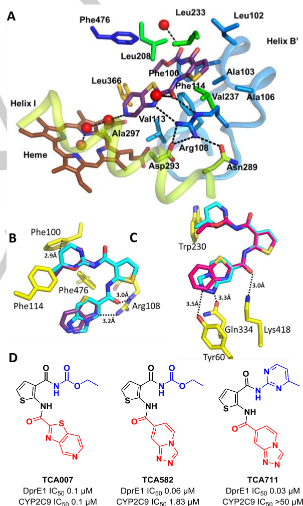
Figure 4. Crystal structure of CYP2C9 with TCA007. A. Key interactions exhibited by TCA007 (violet carbons) in the CYP2C9 active site (PDB: 5W0C). Amino acid side-chains that contact TCA007 are rendered as sticks. The red spheres are water molecules, and the dashed lines depict H-bonds. B. and C. Modeling TCA711 (cyan) in the CYP2C9 structure (overlap with TCA007 in violet) (B) and DprE1 structure (overlap with TCA1 in magenta) (C). D. SAR optimization strategy for TCA1.
