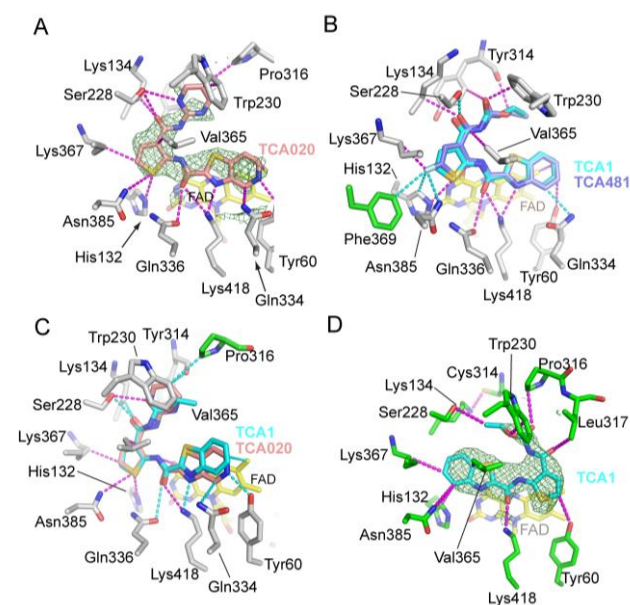
Figure 2. Non-covalent interactions of TCA inhibitors with DprE1. (A) Inhibitor TCA020 (pink) with non-covalent interactions indicated in dashed lines (magenta). The unbiased F_o - F_c density map (contoured at 2.5 \sigma ) was calculated with model phases prior to incorporation of the ligand in the structural model. Protein residues are shown in grey sticks, FAD in yellow sticks. (B, C) Superposition of TCA1 with the inhibitors TCA481 and TCA020, respectively. Dashed lines in cyan indicate new or shortened non-covalent interactions compared to the TCA1:wt-DprE1 complex (see Figure S1 for contact distances). Protein side chains in green indicate amino acids that - in TCA1:wt-DprE1 - fall outside the 4 Å contact radius. (D) The flipped orientation of TCA1 (cyan) in the DprE1-Y314C active site.
