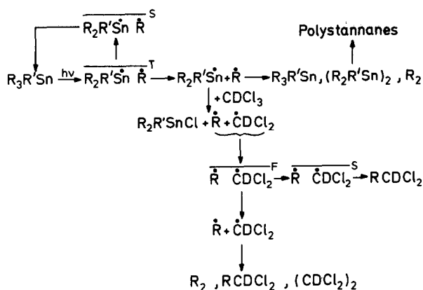
Fig. 3. Reaction scheme for the photochemical decomposition of \text{R}_3\text{R}'\text{Sn} ( \text{R} = \text{CH}_2\text{Ph} , \text{R}' = \text{Me} ).
