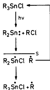
Fig. 5. Stannylene mechanism of (\text{PhCH}_2)_3\text{SnCl} photolysis ( \text{R} = \text{CH}_2\text{Ph} ).
