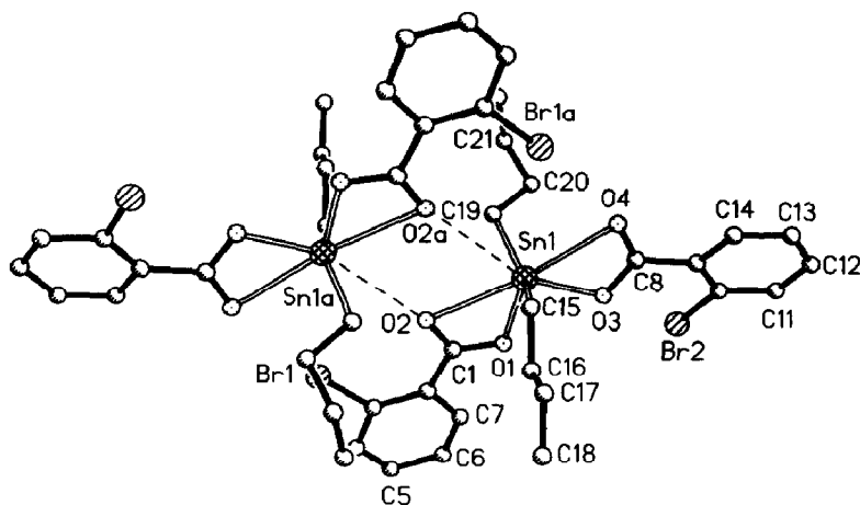
Fig. 1. Structure of di- n -butyltin di- o -bromobenzoate. Selected bond distances and angles: Sn(1)–O(1) 2.095(5), Sn(1)–O(2) 2.608(5), Sn(1)–O(3) 2.097(4), Sn(1)–O(4) 2.617(5), Sn(1)···O(2a) 3.451(5), Sn(1)–C(15) 2.110(7), Sn(1)–O(19) 2.112(7) Å; O(1)–Sn(1)–O(2) 53.8(2), O(2)–Sn(1)···O(2a) 68.9(2), O(2a)···Sn–O(4) 108.2(2), O(4)–Sn(1)–O(3) 53.6(2), O(3)–Sn(1)–O(1) 81.9(2), C(15)–Sn–C(19) 140.5(3)°.
