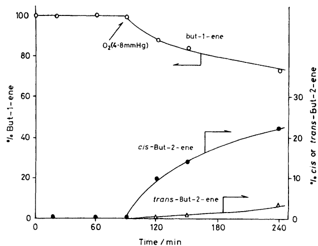
FIGURE. Effect of oxygen on the isomerization of but-1-ene on K 2 CO 3 11.7 wt%-carbon at room temperature (but-1-ene: 186.9 mmHg).
