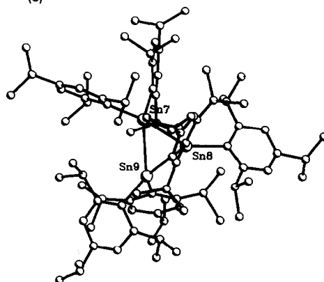
ALKYL TRIMER (c)
